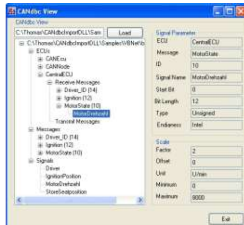
Application using the CANdbc Import DLL
